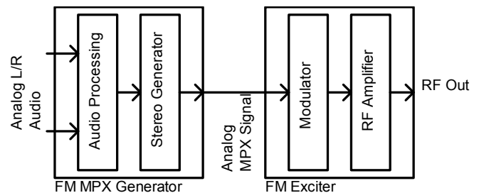
FIG 3 FM SIGNAL PROCESSING CHAIN
