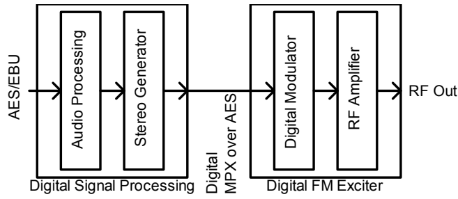
FIG 4 ALL DIGITAL FM SIGNAL PROCESSING CHAIN
